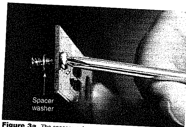
Figure 3a. The spacer washer goes between the azimuth encoder board and the top baseplate of the Dobsonian base.
