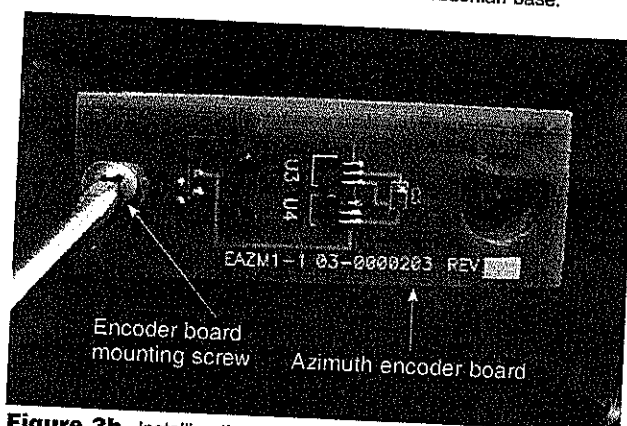
Figure 3b. Installing the azimuth encoder board. Line up the large hole in the encoder board with the central hole in the top baseplate.
