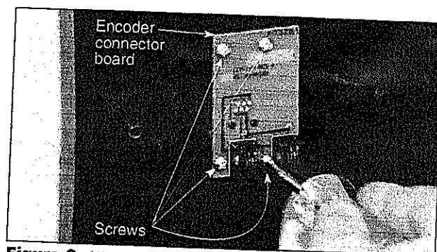
Figure 6. Attaching the encoder connector board.
