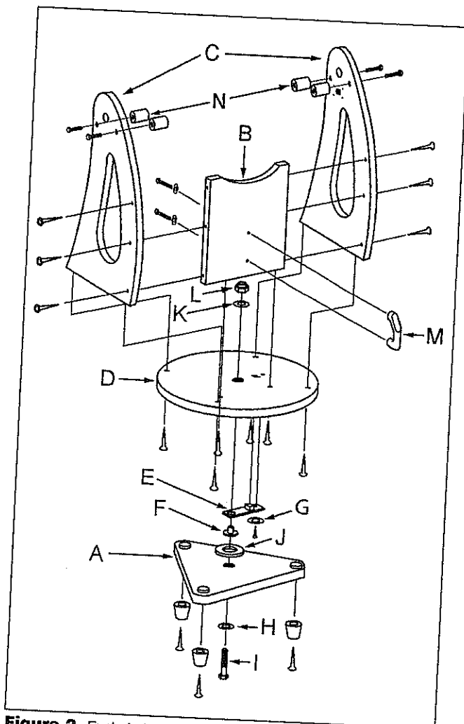
Figure 2. Exploded view of the XTi IntelliScope Dobsonian base.
