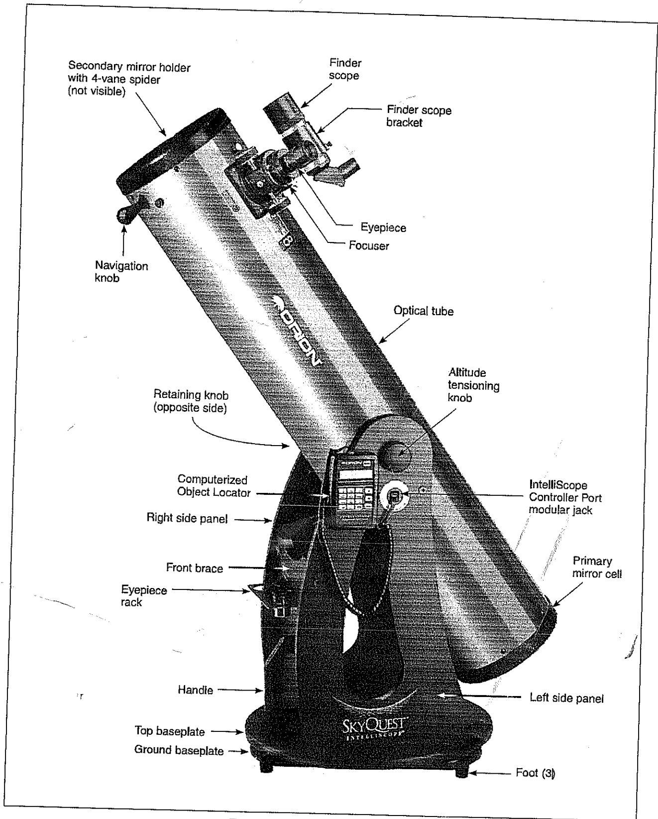
Figure 1. The SkyQuest XT8 IntelliScope
