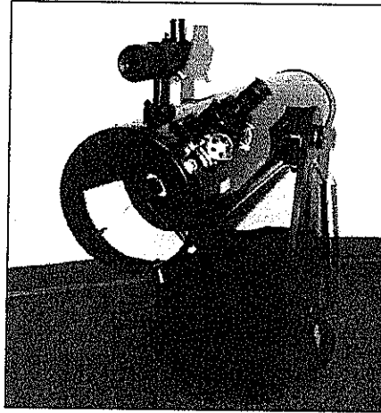
Figure 20. The SkyQuest XTi IntelliScope properly set up for collimation. Note the white paper placed across from the focuser, and the level angle of the optical tube. Ideally, the telescope should be pointing at a white wall.
