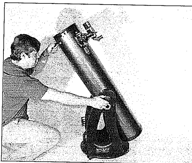
Figure 15. Adjust the tensioning knob until the altitude balance is just right. The telescope should move easily in altitude without drifting when you let go.
