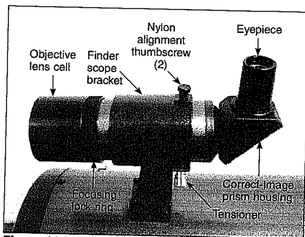
Figure 12a. The 9x50 right-angle correct-image finder scope and bracket (6x30 for the XT6i).
