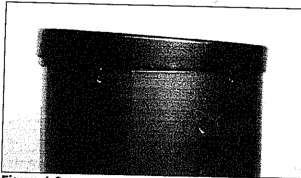
Figure 1.6. Lower the assembled mirror cell onto the tube so one side of the end ring is seated on the tube edge. The threaded attachment holes in the end ring should also be lined up with the through holes in the end of the tube.
