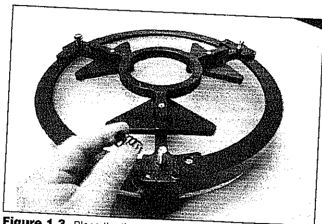
Figure 1.3. Place the three springs on the exposed threaded shafts of the mirror cell.
