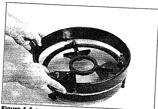
Figure 1.4. Lower the rear end ring onto the mirror cell so that the threaded shafts pass through the end ring, and the end ring rests on the springs.
